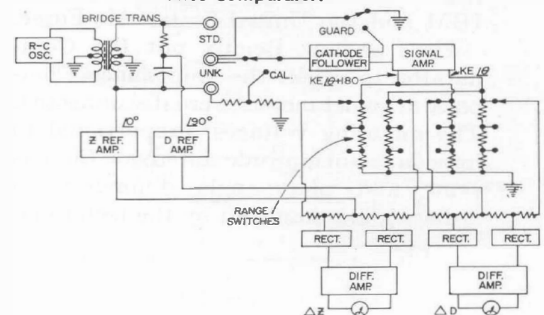
Figure 1. Block diagram of the Type 1605-A Impedance Comparator.
