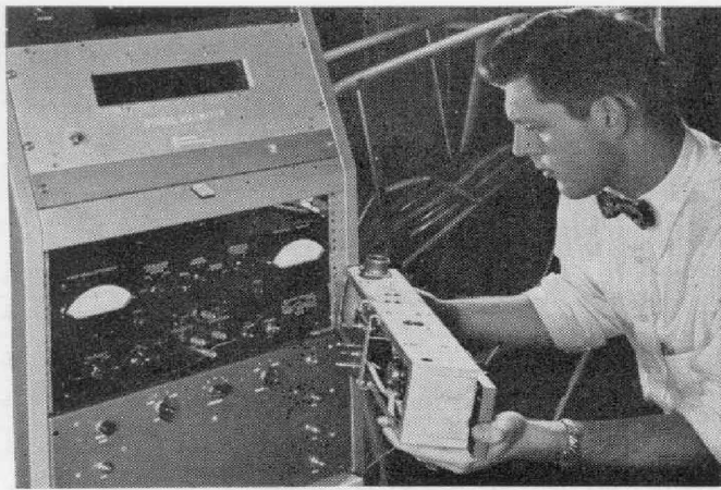
Figure 3. Inland Testing Laboratories use the Impedance Comparator in an automated instrumentation system for environmental reliability tests on capacitors.
