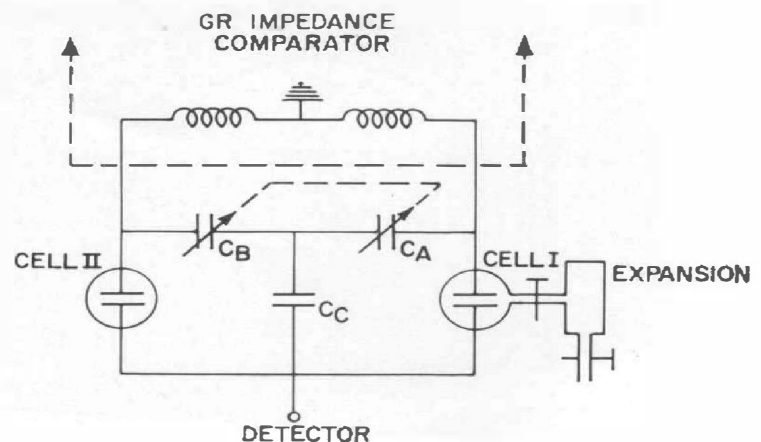
Figure 4. Circuit used for measurement of small changes in dielectric constant.
